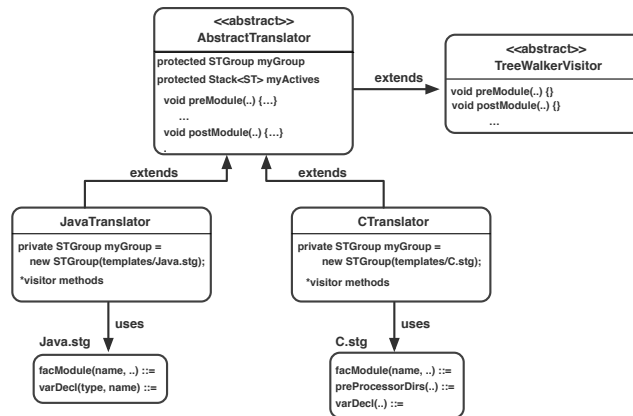
Figure 8. A translation hierarchy. Each concrete subclass of the abstract translator has an accompanying, dedicated Stringtemplate group file containing all templates tailored to the target language of the class.
